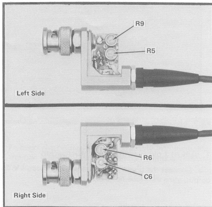
Fig. 9. Location of high-frequency compensation adjustments.
