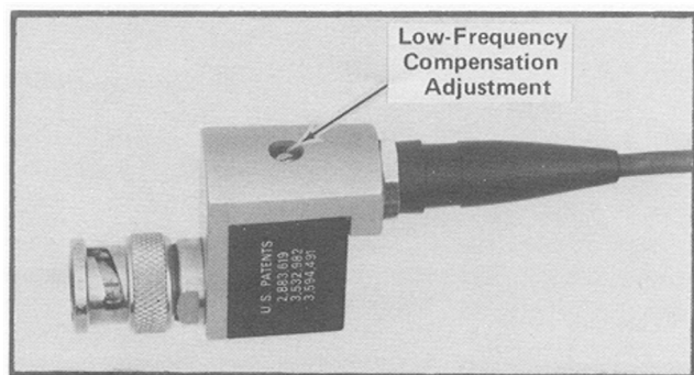
Fig. 7. Location of probe low-frequency compensation adjustment.
