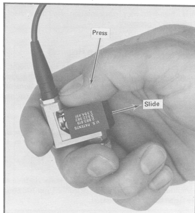
Fig. 6. Removal of compensation box cover.
